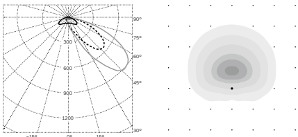
TP08 (ewoLightTile) Asymmetric Extra Forward
