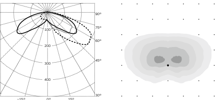
TS11 (ewoLightTile) Asymmetric Side and Forward Throw
